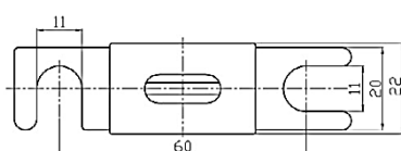
ANL fuse
